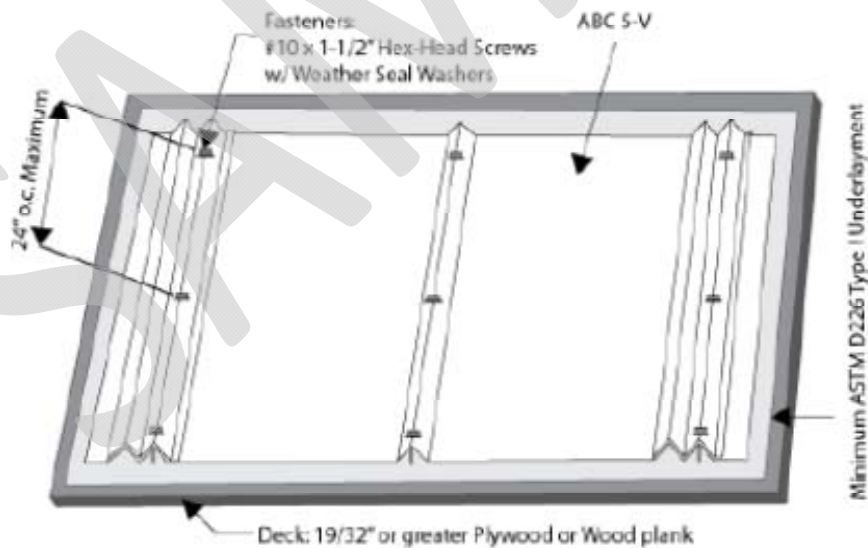
Figure 2 Anchorage Detail B
